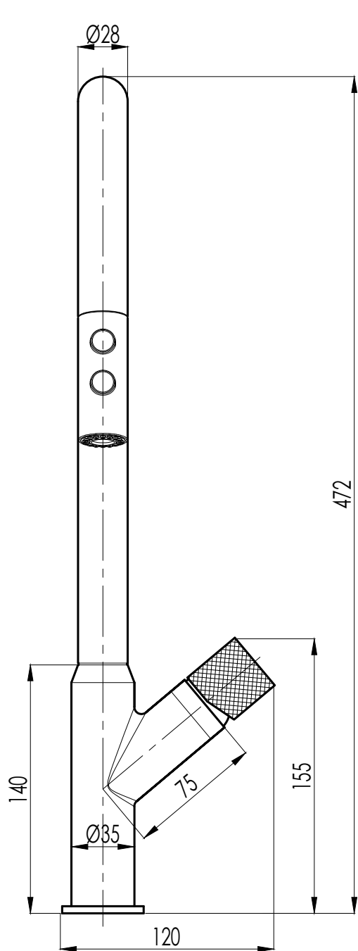
Front View
