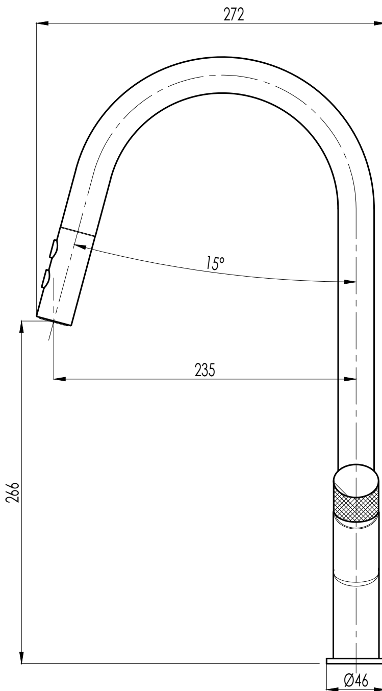
Side View
